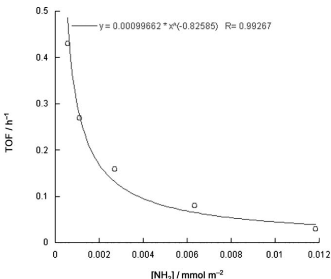
Figure 5. Fitted curve of base activity versus base concentration on the APMSNN surface (reaction conditions were the same as those used in Table 1).
