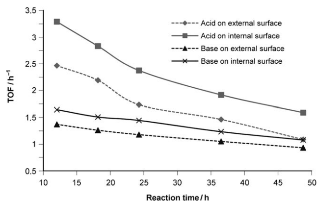
Figure 4. Turnover frequency of the acid and base catalysts that are located on either the internal or external surfaces of SAMSNN-AP and APMSNN-SA.
