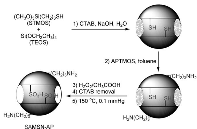
Figure 1. Syntheses of bifunctional mesoporous silica nanoparticles having sulfonic acid groups on the internal surface and organic amine groups on the external surface.
